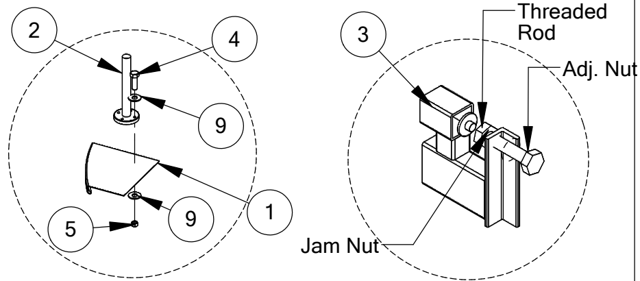
DETAIL B Tension Adjustment View
