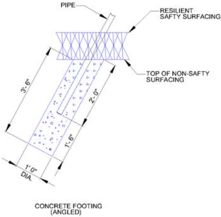
Diagram: Permanent Installation
