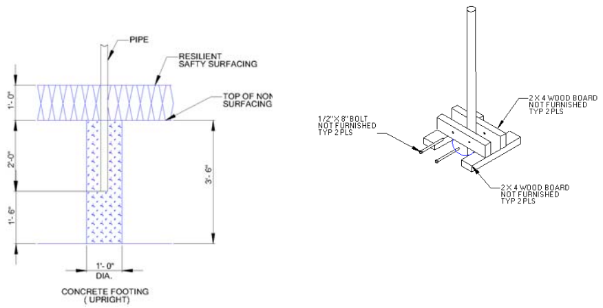
Diagram: Suggested Bracing Method
