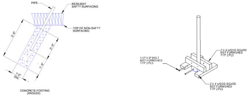
Diagram: Suggested Bracing Method
