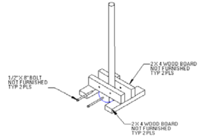
Detail: Suggested Bracing Method
